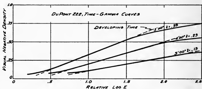
FIG. 6. Dupont 222. Time-gamma characteristics in special negative developer.
